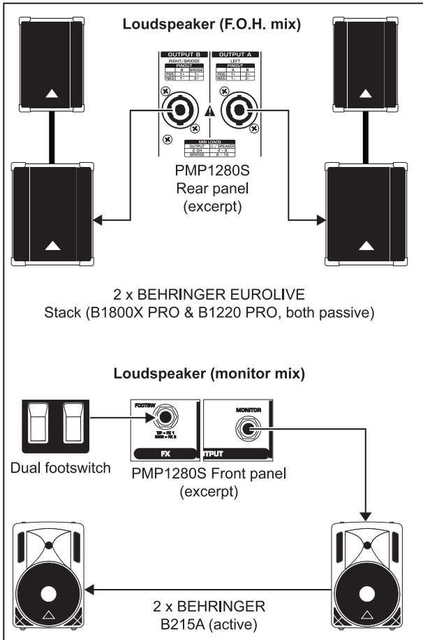
Fig. 5.1: EUROPOWER mixer as a stereo amplifier (example)
