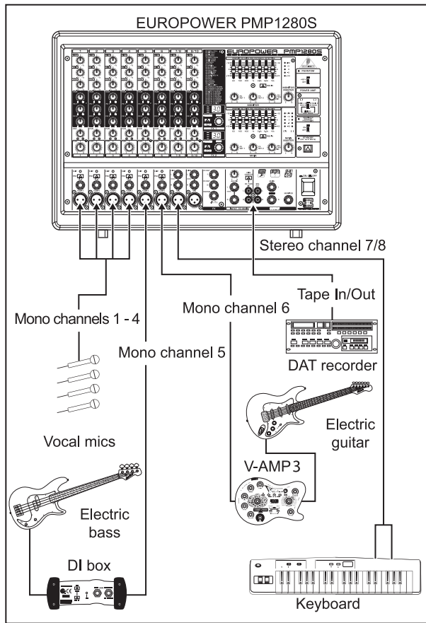
Fig. 5.3: Standard set-up (example)
