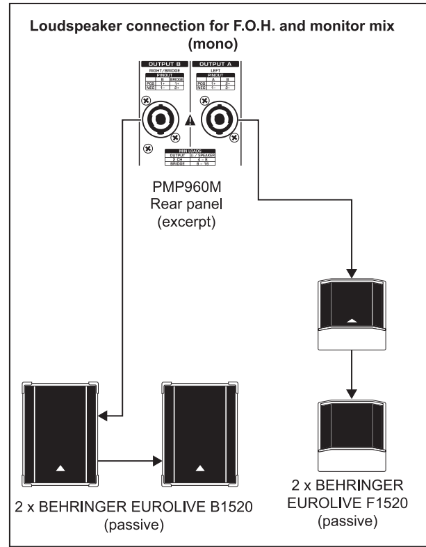
Fig. 5.2: EUROPOWER as a dual mono amplifier (example)
