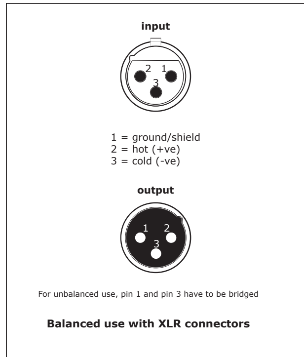
Fig. 4.3: XLR connectors
