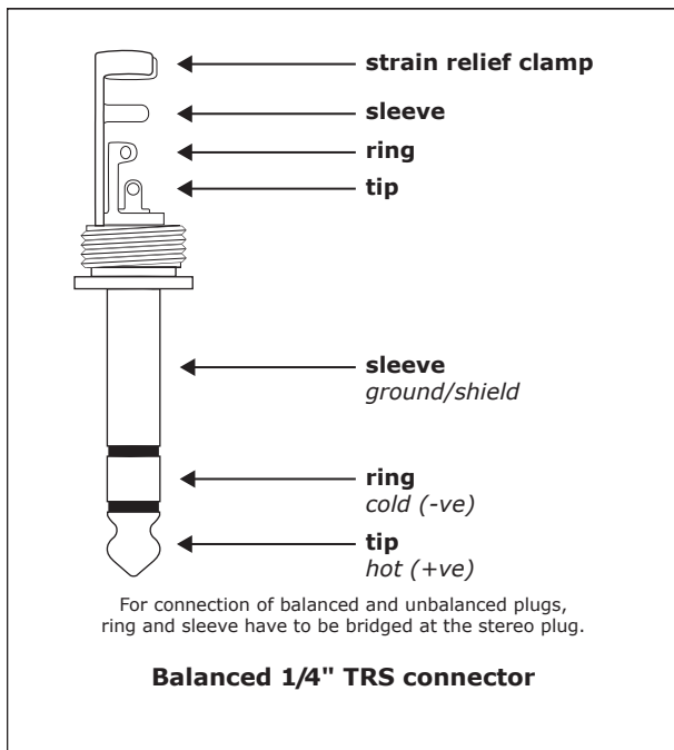
Fig. 4.2: 1/4" TRS connector
