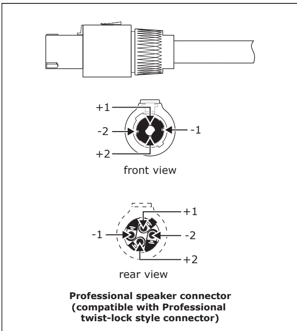
Fig. 4.6: Professional twist-lock style connector
