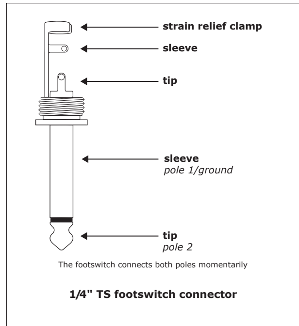
Fig. 4.4: 1/4" TS connector for footswitch
