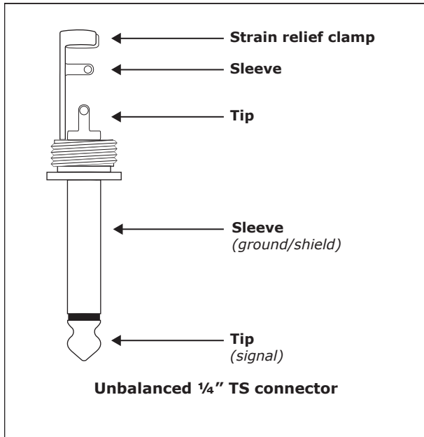
Fig. 4.1: 1/4" TS connector
