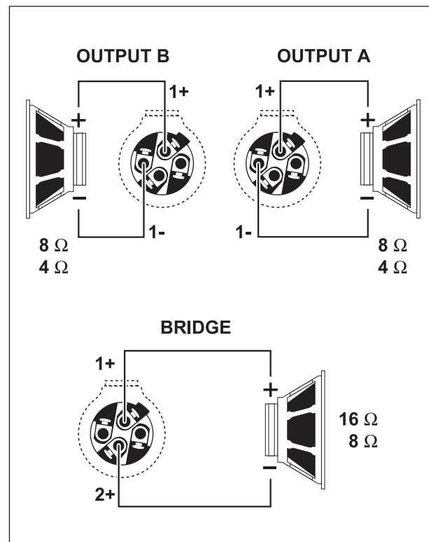
Fig. 4.7: Connector assignment
